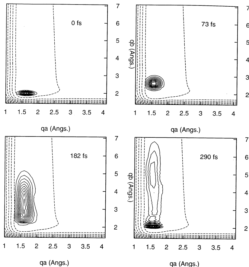
Fig. 6. Time evolution of the \Psi_{1A}(q_a, q_b, t) (solid line) wavepacket on the V_{1A}(q_a, q_b) (dashed line) potential as a function of q_a = [\text{Mn-H}] and q_b = [\text{Mn-CO}_{ax}] .
