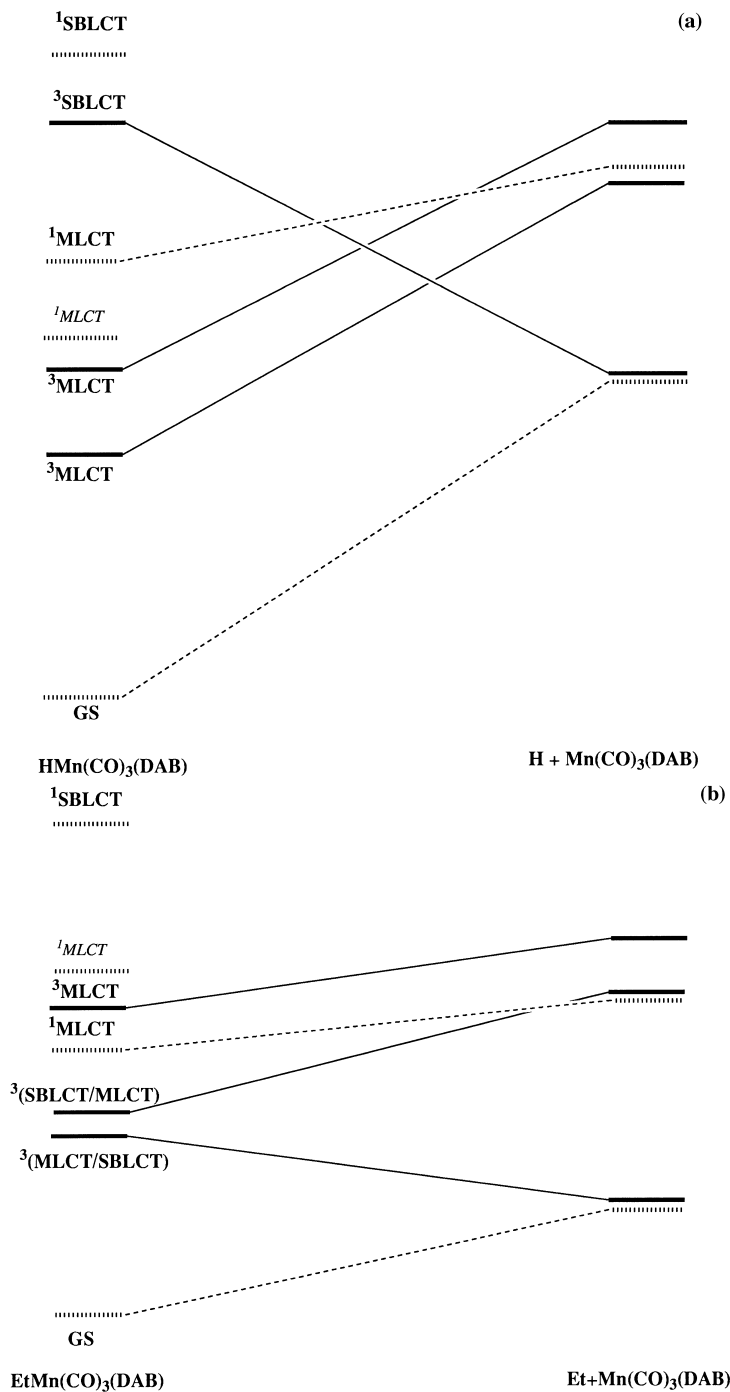
Fig. 7. State correlation diagrams connecting the low-lying electronic states of (a) Mn(H)(CO) 3 (DAB) and (b) Mn(Et)(CO) 3 (DAB).
