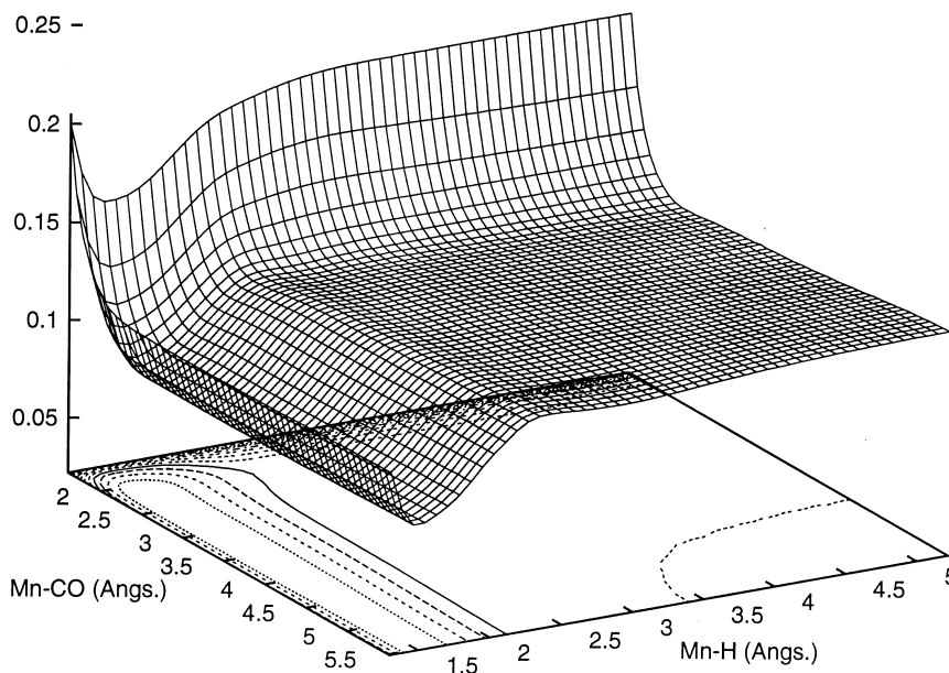
Fig. 5. Two-dimensional PES V_{c^1A'}(q_a, q_b) associated with the c^1A' MLCT excited state used in the simulation of the 2D photodissociation dynamics.
