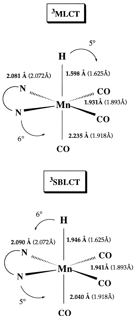
Fig. 2. Gradient/CASSCF optimized geometries of the lowest ^3\text{MLCT} and ^3\text{SBLCT} excited states in \text{Mn}(\text{H})(\text{CO})_3(\text{DAB}) (the electronic ground state bond distances are given in parentheses).
