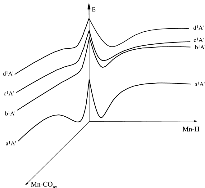
Fig. 3. Sets of CASSCF/MRCI potential energy curves calculated for the low-lying singlet states as a function of the Mn–H and Mn–CO ax bonds elongations in Mn(H)(CO) 3 (DAB).
